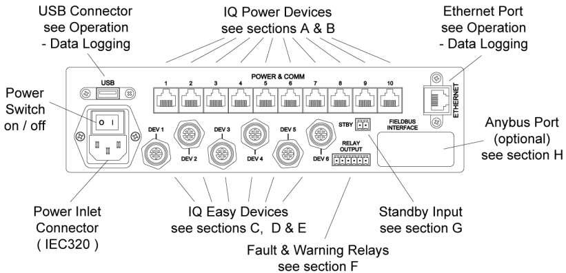
Figure 13. IQ Power Control Station Connectors
