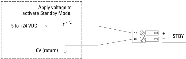
Figure 16. IQ Power Control Station STBY (Standby Schematic)
