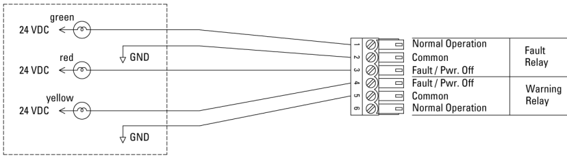
Figure 14. IQ Power Control Station Relay Output (Typical Light Tree Schematic)
