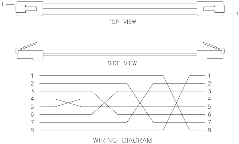
Figure 1. IQ Power Crossover Modular Cable (black)
